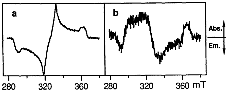
Figure 3 TR-ESR spectra of a) \text{TTPH}_2 and b) o,o\text{-C}_3(\text{TTP})_2\text{CuH}_2 in toluene at 77K.
